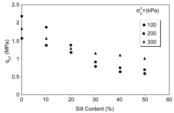
Figure 5. Variation in normalized cone penetration resistance, q_{cl} (MPa) with silt content.
