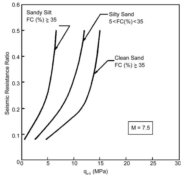
Figure 4. CPT-Based liquefaction-potential relationships for sand-silt mixtures and M=7.5 earthquakes [2].
