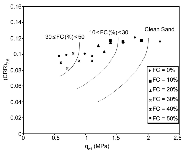
Figure 7. Proposed correlations between cyclic resistance ratio for 7.5-magnitude earthquake, (CRR)_{7.5} and normalized cone penetration resistance, q_{c1} for sand-silt mixtures.
