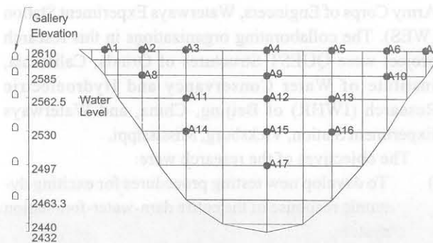
Figure 3. Accelerometers mounted on dam crest and in galleries.
