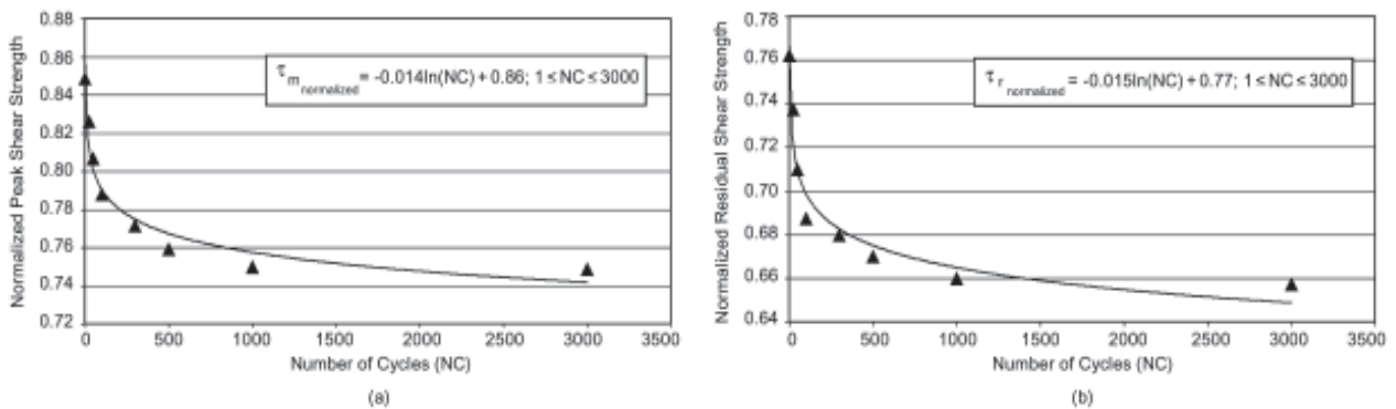
Figure 8. Logarithmic trends for decrease of normalized shear strength (normalized by \sigma_3 ) with number of cycles; a) Peak values ; b) Mean residual values.
