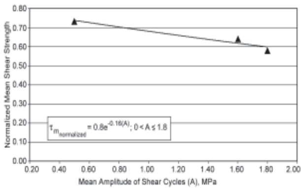
Figure 10. Sharp decrease of shear strength (normalized by \sigma_3 ) due to increase of loading amplitude.
