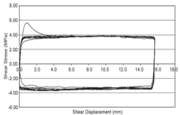
Figure 14. Shear stress-shear displacement curve for saw-tooth samples during 10 cycles in 6.5MPa normal stresses.
