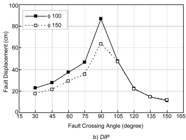
Figure 8. Allowable fault displacement vs. fault crossing angle.
