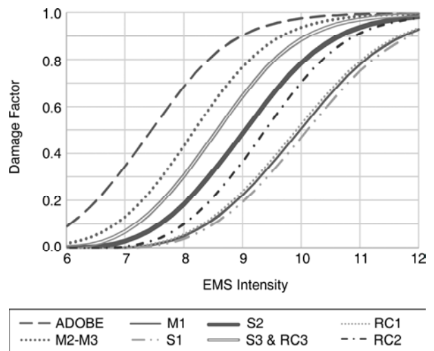
Figure 7. Calibrated vulnerability curves according to EMS-98.
