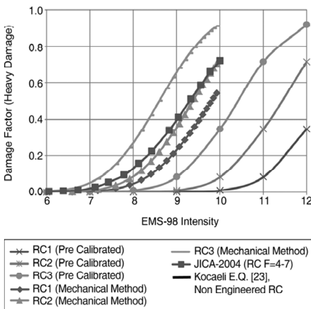
Figure 6. Damage curves for R/C buildings according to mechanical modeling, preliminary EMS-98 parameters, JICA-2004 and empirical data of Kocaeli 1999 earthquake [23].
