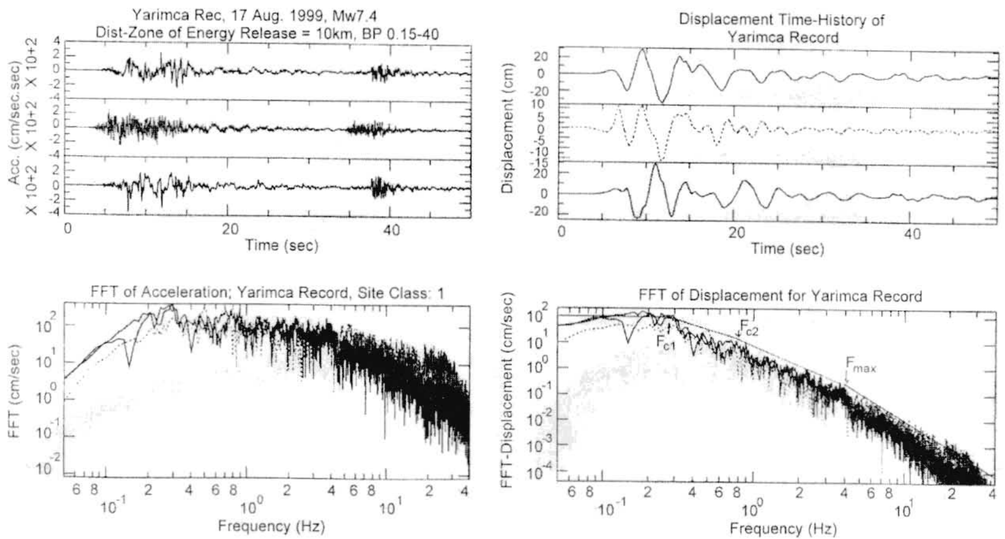
Figure 9. The Yarimca record; a) the filtered accelerogram, b) the FFT of accelerations, c) the displacement time-history and d) the FFT of displacement, where the f_{c1} , f_{c2} and f_{max} are shown in the figure. The upper and lower figures are the horizontal components and the middle one corresponds to the vertical component.
