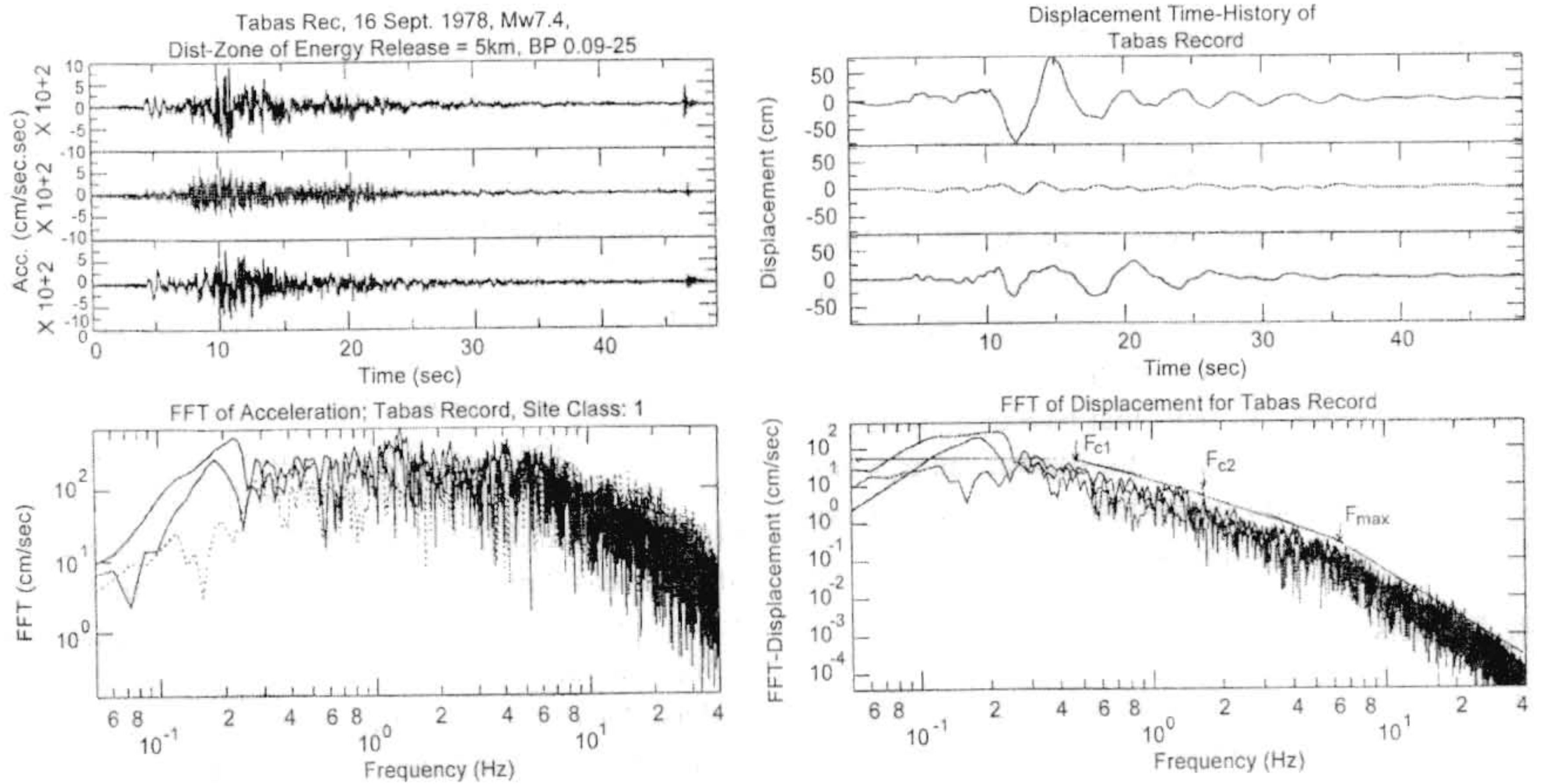
Figure 5. The Tabas record; a) the filtered accelerogram, b) the FFT of accelerations, c) the displacement time-history and d) the FFT of displacement, where the f_{c1} , f_{c2} and f_{max} are shown in the figure. The upper and lower figures are the horizontal components and the middle one corresponds to the vertical component.
