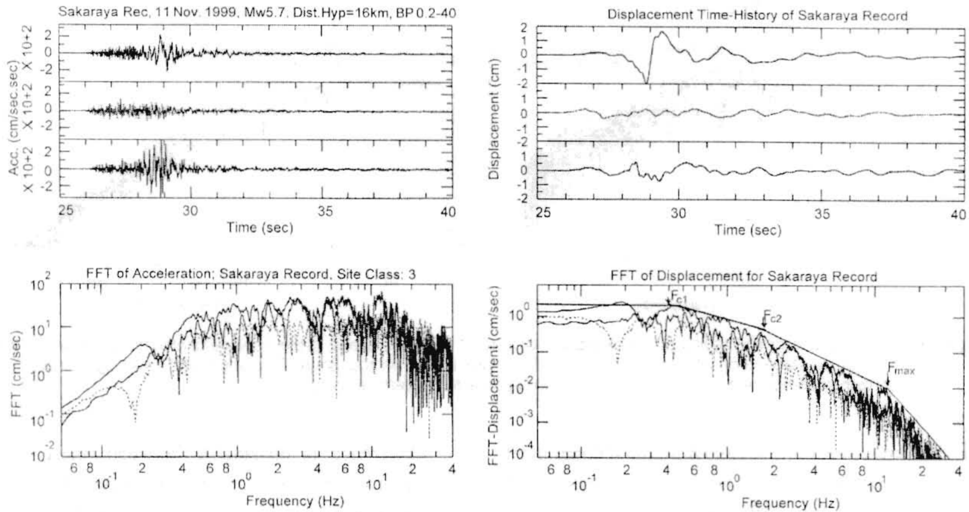
Figure 11. The Sakaraya (Adapazari) record; a) The filtered accelerogram, b) the FFT of accelerations, c) the displacement time-history and d) the FFT of displacement, where the f_{c1} , f_{c2} and f_{max} are shown in the figure. The upper and lower figures are the horizontal components and the middle one corresponds to the vertical component.
