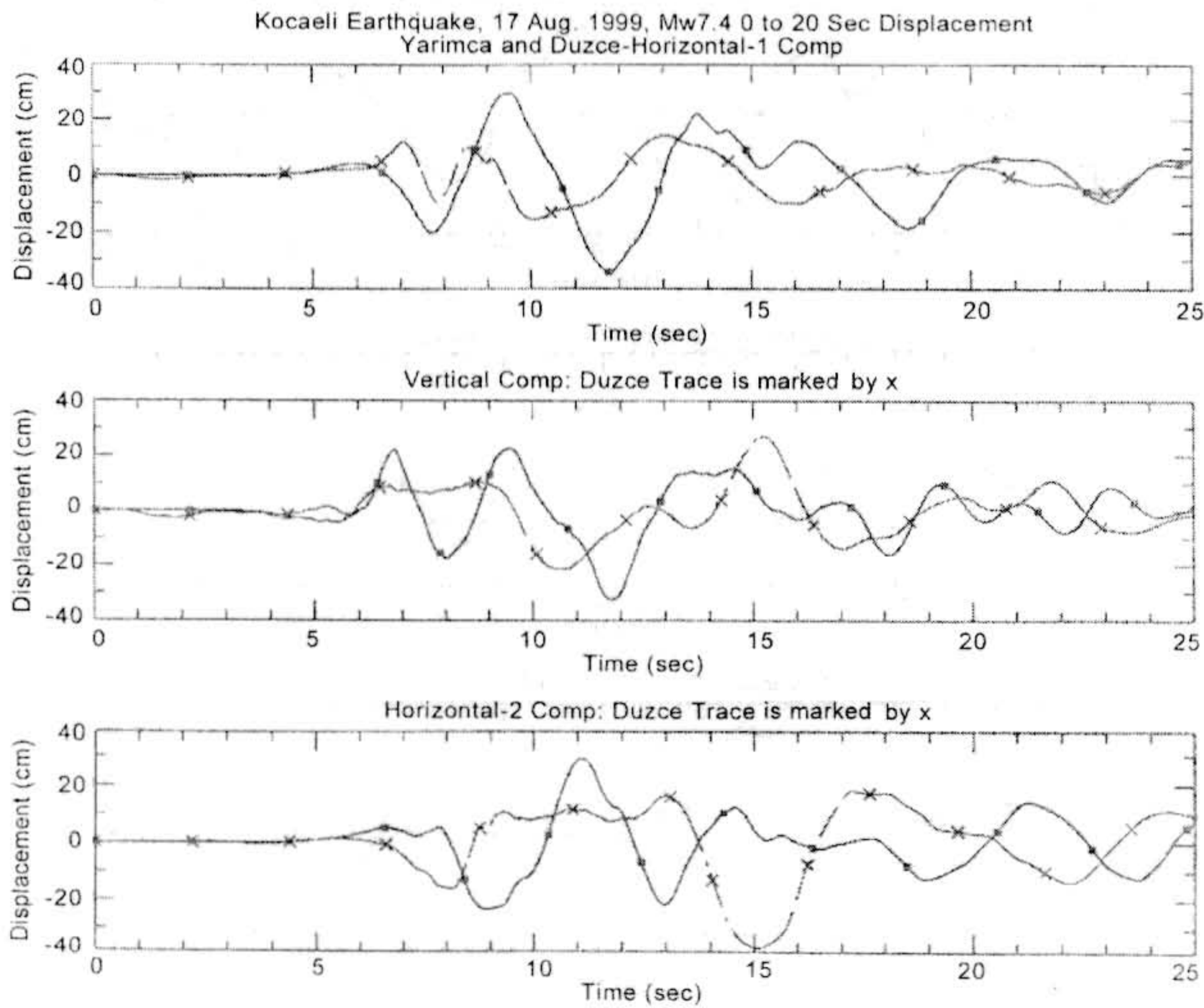
Figure 17. The displacement time-histories are compared for Yarimca and Duzce records for different components: the upper and lower are the horizontal components and the middle one is the vertical component (the Duzce traces are shown in dashed lines).
