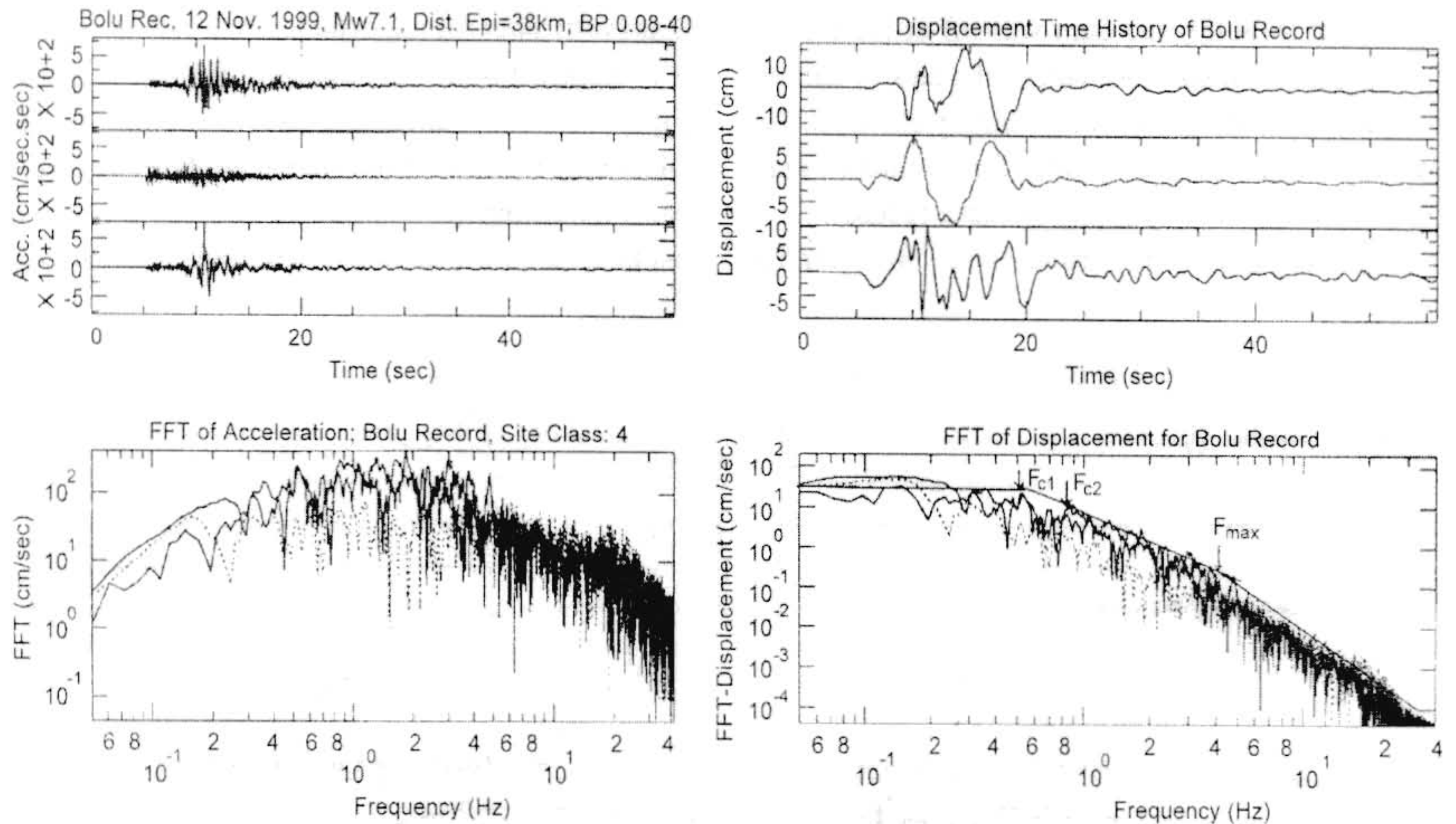
Figure 13. The Bolu record; a) The filtered accelerogram, b) the FFT of accelerations, c) the displacement time-history and d) the FFT of displacement, where the f_{c1} , f_{c2} and f_{max} are shown in the figure. The upper and lower figures are the horizontal components and the middle one corresponds to the vertical component.
