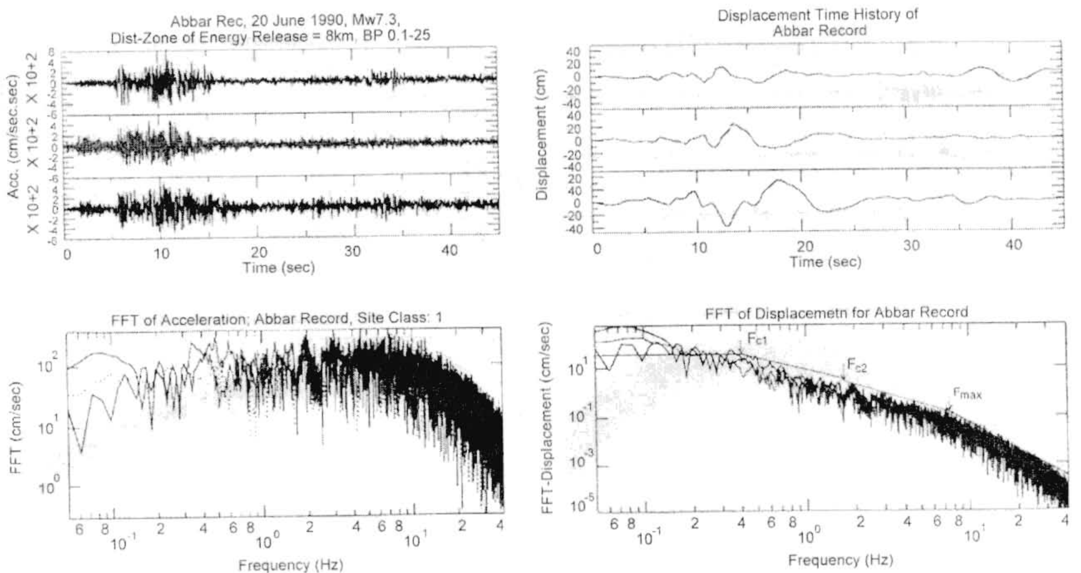
Figure 6. The Abbar record; a) the filtered accelerogram, b) the FFT of accelerations, c) the displacement time-history and d) the FFT of displacement, where the f_{c1} , f_{c2} and f_{max} are shown in the figure. The upper and lower figures are the horizontal components and the middle one corresponds to the vertical component.
