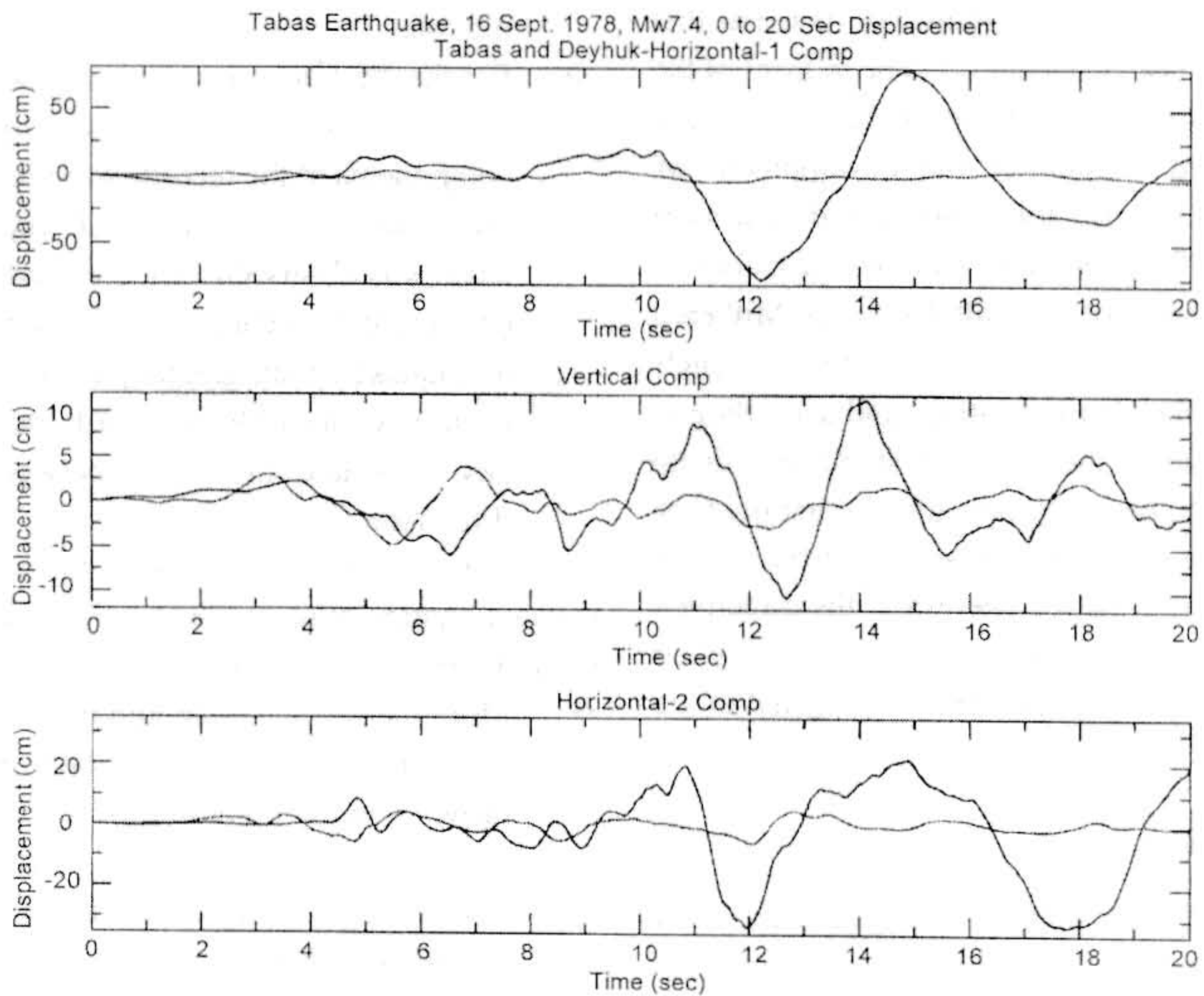
Figure 15. The displacement time-histories are compared for Tabas and Deyhuk records for different components: the upper and lower are the horizontal components and the middle one is the vertical component (the Deyhuk traces are shown with dashed lines).
