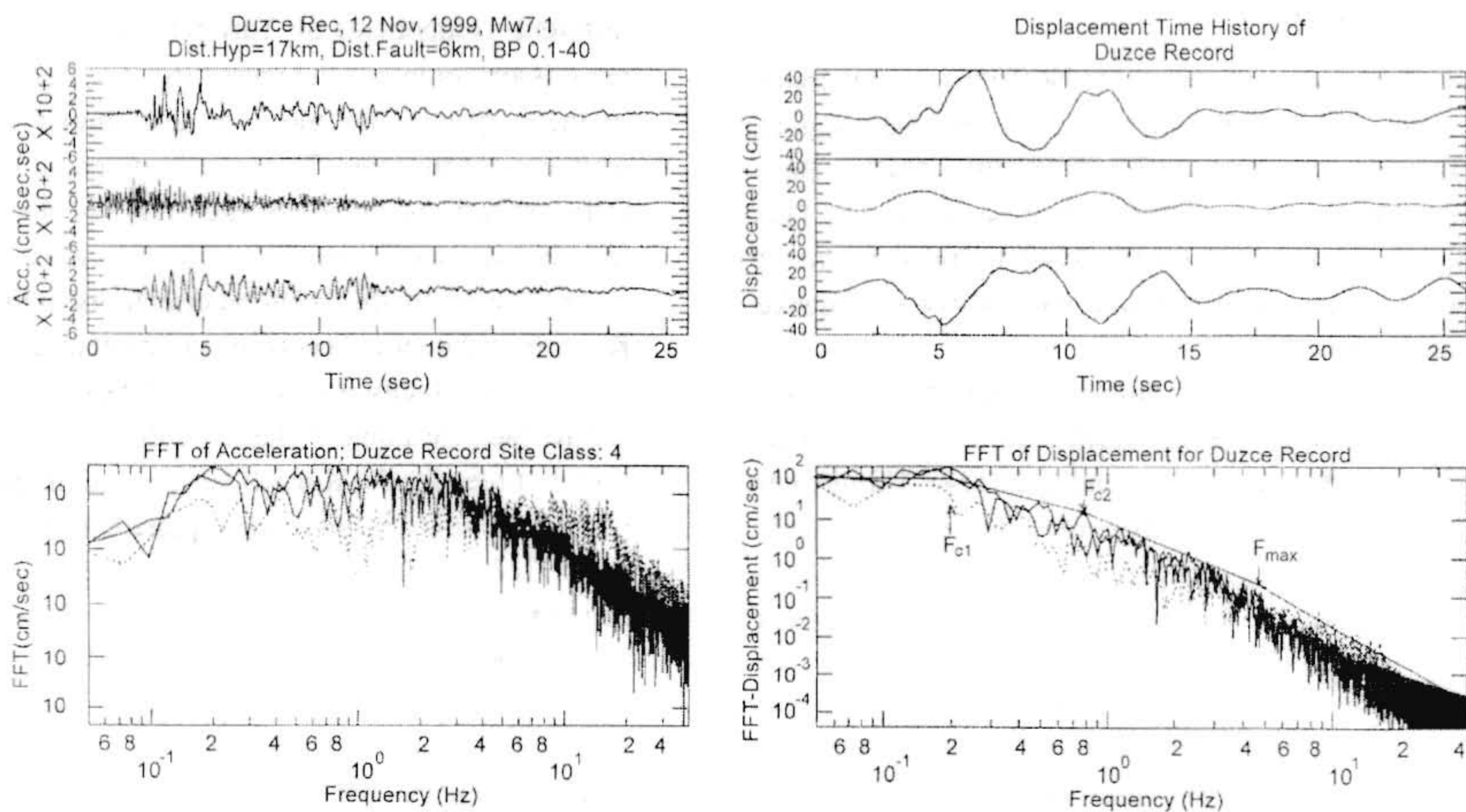
Figure 12. The Duzce record (of 12/11/1999 earthquake); a) the filtered accelerogram, b) the FFT of accelerations, c) the displacement time-history and d) the FFT of displacement, where the f_{c1} , f_{c2} and f_{max} are shown in the figure. The upper and lower figures are the horizontal components and the middle one corresponds to the vertical component.
