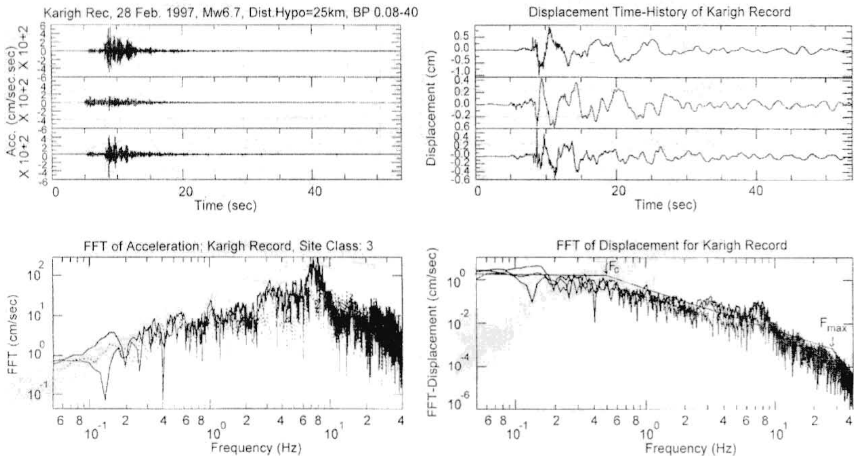
Figure 8. The Karigh record; a) the filtered accelerogram, b) the FFT of accelerations, c) the displacement time-history and d) the FFT of displacement, where the f_{c1} , f_{c2} and f_{max} are shown in the figure. The upper and lower figures are the horizontal components and the middle one corresponds to the vertical component.
