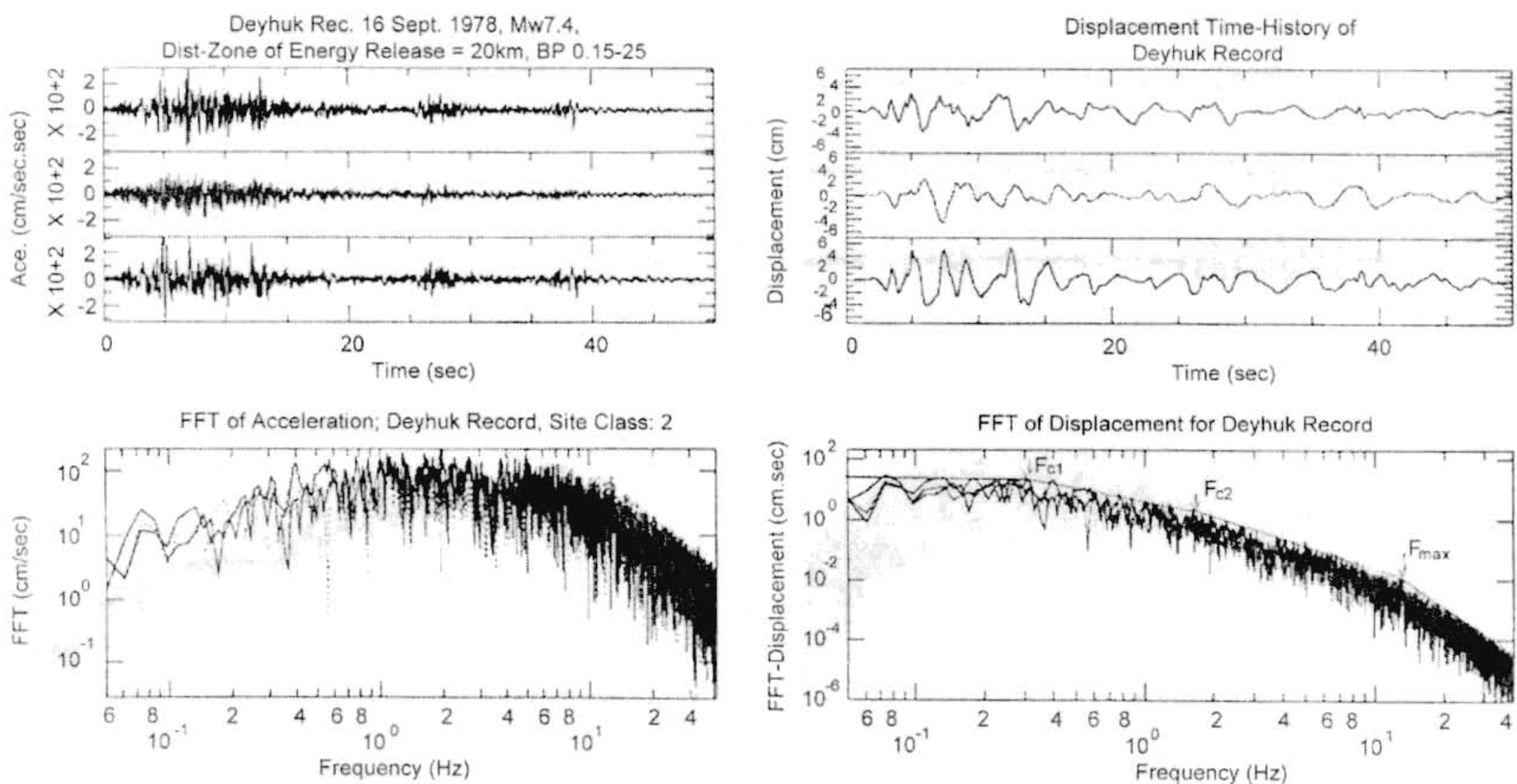
Figure 4. The Deyhuk record; a) The filtered accelerogram, b) The FFT of accelerations, c) The displacement time-history and d) The FFT of displacement, where the f_{c1} , f_{c2} and f_{max} are shown in the figure. The upper and lower figures are the horizontal components and the middle one corresponds to the vertical component.
