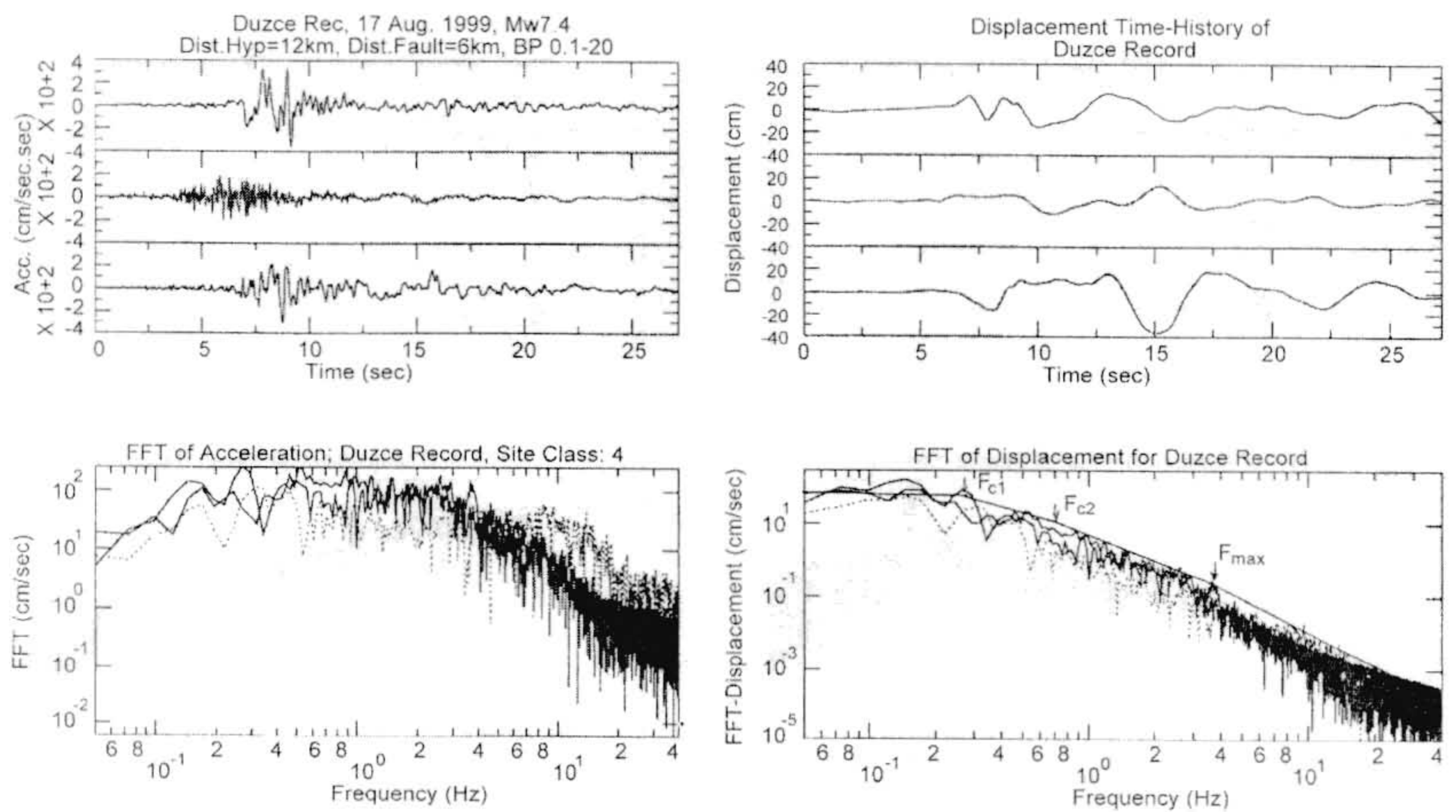
Figure 10. The Duzce record (of 17/08/1999 earthquake); a) The filtered accelerogram, b) the FFT of accelerations, c) the displacement time-history and d) the FFT of displacement, where the f_{c1} , f_{c2} and f_{max} are shown in the figure. The upper and lower figures are the horizontal components and the middle one corresponds to the vertical component.
