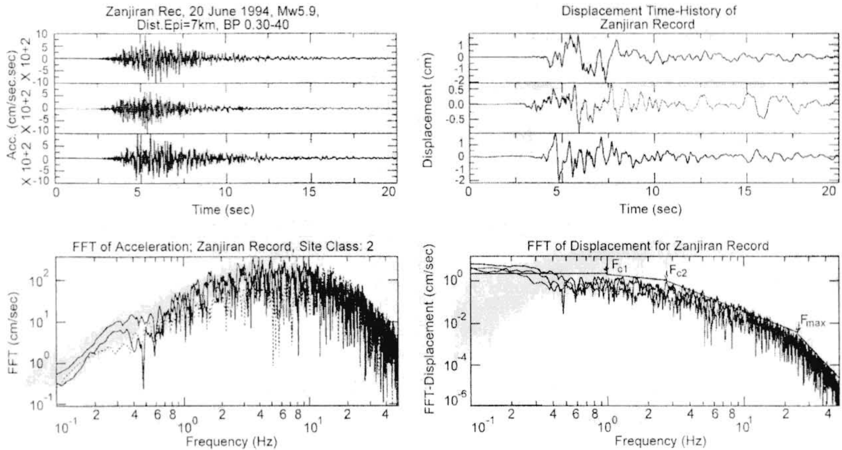
Figure 7. The Zanjiran record; a) the filtered accelerogram, b) the FFT of accelerations, c) the displacement time-history and d) the FFT of displacement, where the f_{c1} , f_{c2} and f_{max} are shown in the figure. The upper and lower figures are the horizontal components and the middle one corresponds to the vertical component.
