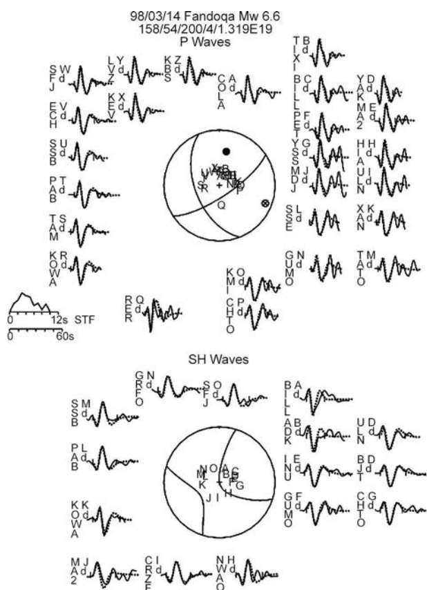
Figure 4. Minimum misfit solution for the 14 March 1998 earthquake in Gowk fault, see Table (2), showing P (top) and SH (bottom) observed (solid) and synthetic (dotted) waveforms. Waveforms for each station are arranged azimuthally around the focal spheres. Station positions on focal spheres are identified by capital letters and arranged clockwise starting from north. STF is the source time function. Vertical ticks on the seismograms indicate the inversion window. Numbers beneath the header line are strike, dip, rake, centroid depth (km) and scalar moment (N.M). Stations were weighted according to azimuthally density and then S seismograms weights were halved to compensate for their larger amplitudes. P and T axes are represented by a black and white dot.
