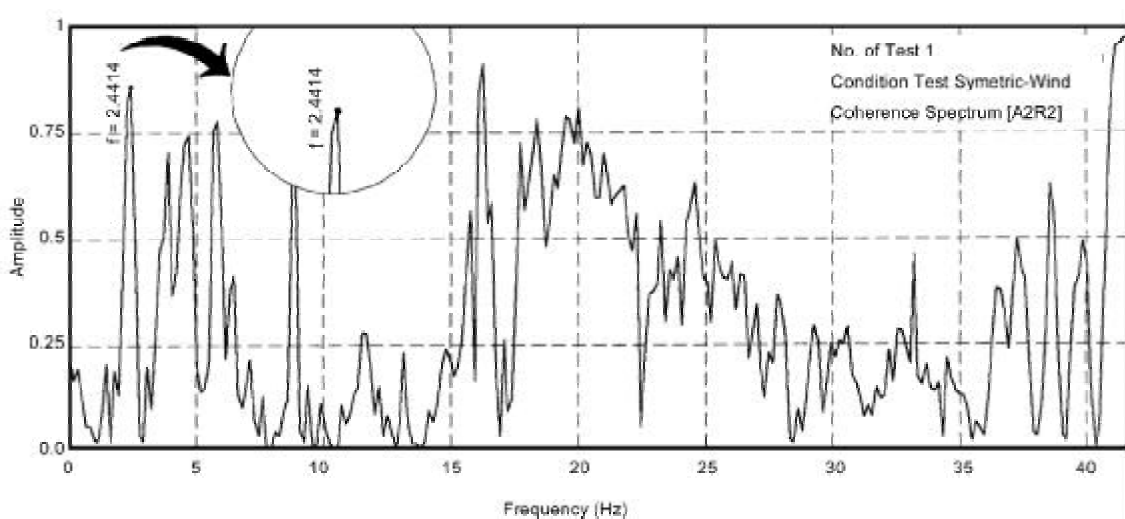
Figure 6e. Coherence spectrum between station [A2 and R2] at crest midpoint (Symmetric wind condition-Shahid-Rajae dam).
