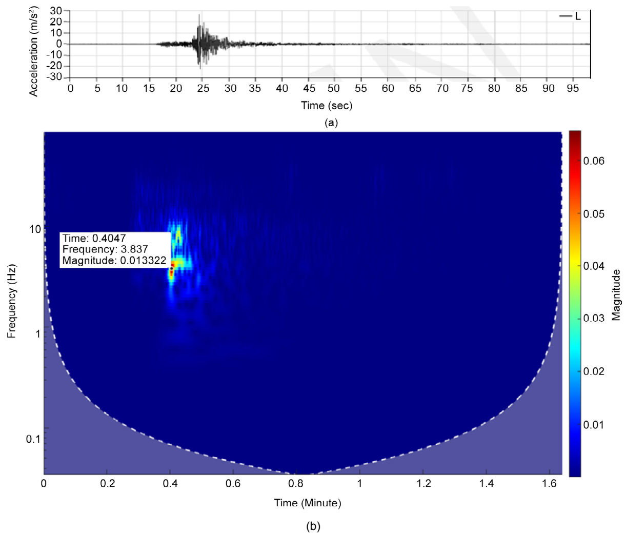
Figure 4. (a) The accelerogram recorded for the far-field of the 2020 Mosha earthquake at the Tehran 303 station (Shahid Rajaei University, 57 km distance); (b) The wavelet transform of the accelerogram recorded for the far-field of the 2020 Mosha earthquake at the Tehran 303 station (Shahid Rajaei University, 57 km distance).
