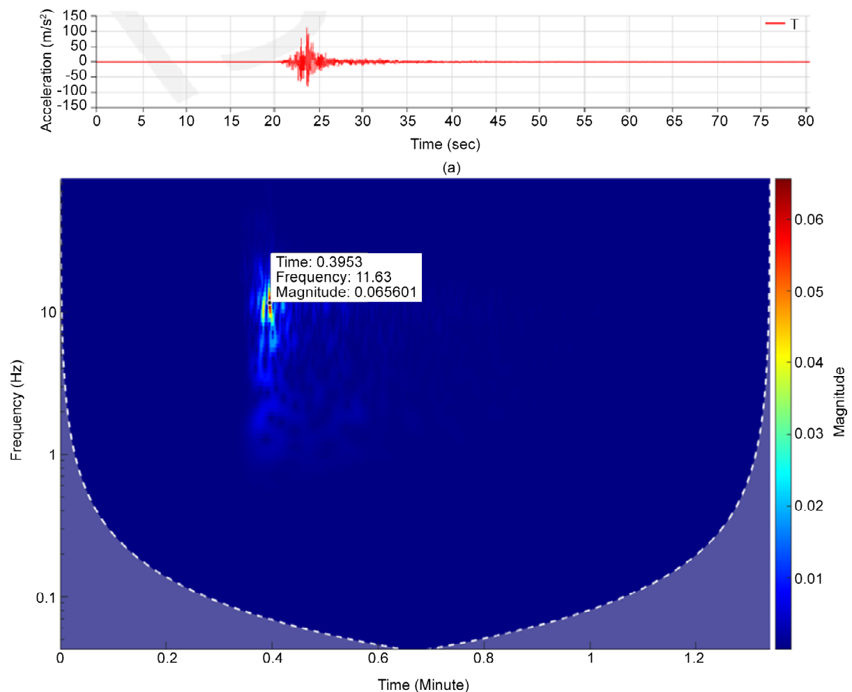
Figure 2. (a) The accelerogram recorded for the near-field of the 2020 Mosha earthquake at the Mosha-3 station (13 km distance); (b) The wavelet transform of the accelerogram recorded for the near-field of the 2020 Mosha earthquake at the Mosha-3 station (13 km distance).
