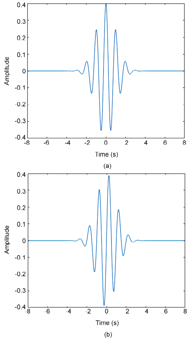
Figure 1. (a) Real part of the complex Morlet wavelet and (b) Imaginary part of the complex Morlet wavelet.
