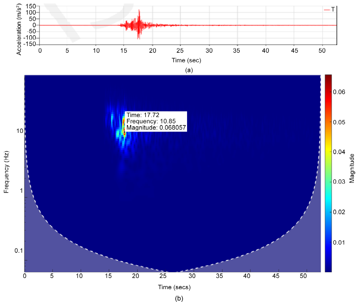
Figure 3. (a) The accelerogram recorded for the medium-field of the 2020 Mosha earthquake at the Rudehen station (22 km distance); (b) The wavelet transform of the accelerogram recorded for the medium-field of the 2020 Mosha earthquake at the Rudehen station (22 km distance).
